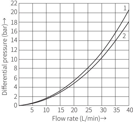
\Delta p - q_v characteristic curve 3/2-way poppet directional valve
