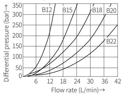
\Delta p - q_v characteristic curve Cartridge throttle
