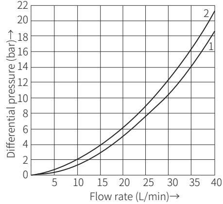
\Delta p - q_v characteristic curve 4/2-way poppet directional valve
